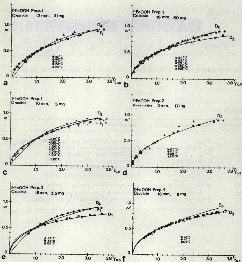
Fig. 6. Isothermal dehydration of 4 samples of \gamma -FeOOH at various temperatures in vacuo. Reduced time representation. The drawn out functions are those of Fig. 5. (a) Preparation 1, crucible 12 mm \varnothing , 31 mg. (b) Preparation 1, crucible 16 mm \varnothing , 50 mg. (c) Preparation 1, crucible 16 mm \varnothing , 5 mg. (d) Preparation 2, crucible 3 mm \varnothing , 17 mg. (e) Preparation 3, crucible 16 mm \varnothing , 3.5 mg. (f) Preparation 4, crucible 16 mm \varnothing , 5 mg.
